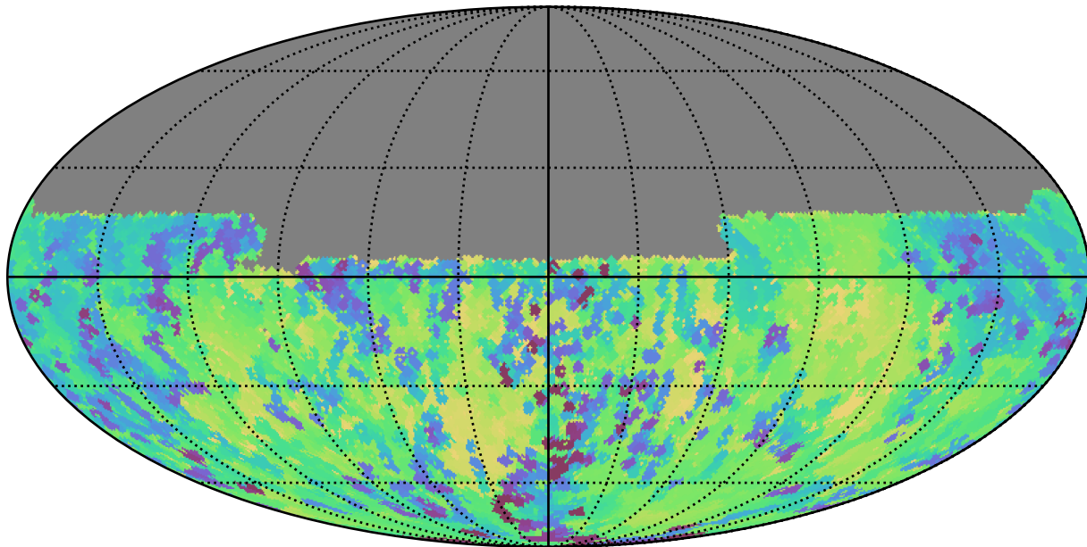
weather_cloudso6v3.4_10yrs Yr 1 y band: Min skyBrightness
