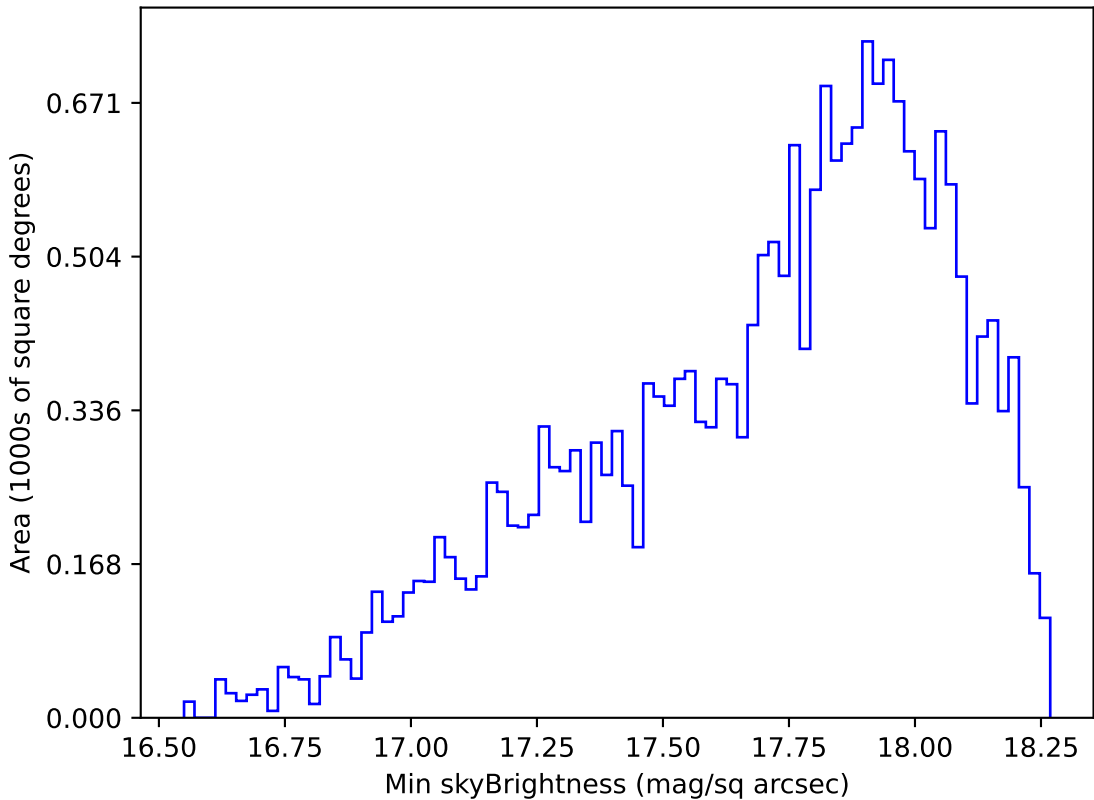
weather_cloudso6v3.4_10yrs Yr 1 y band: Min skyBrightness
