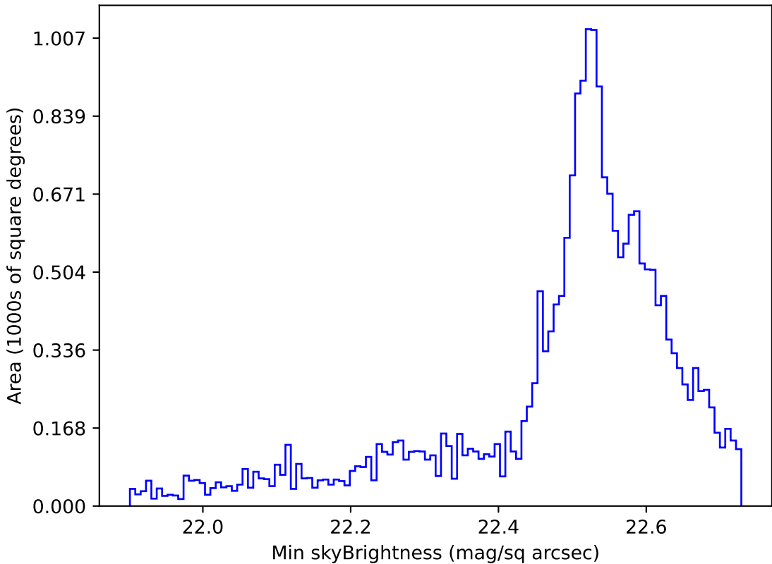
weather_cloudso6v3.4_10yrs Yr 1 u band: Min skyBrightness
