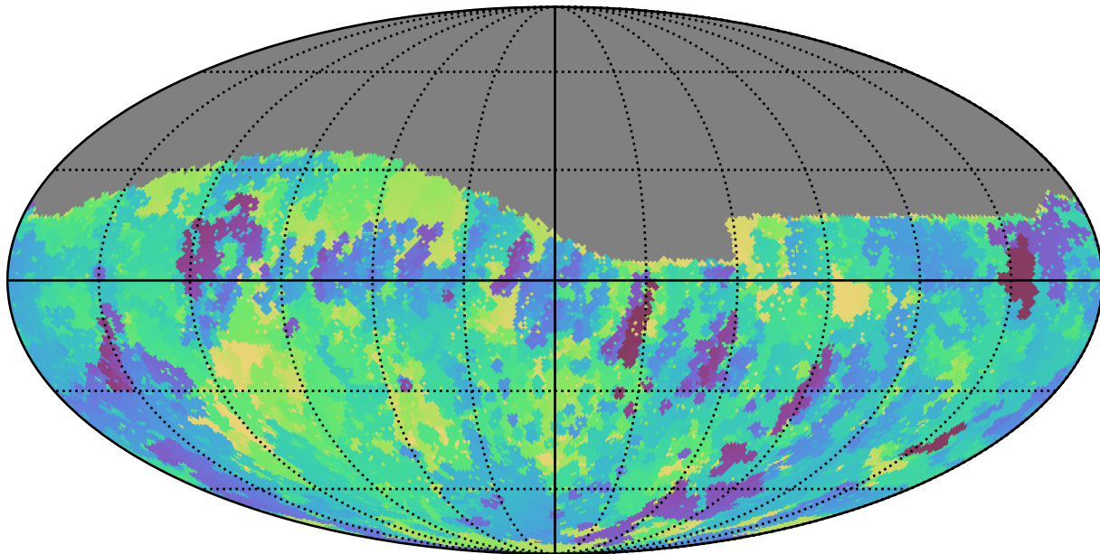
weather_cloudso6v3.4_10yrs Yr 1 r band: Min skyBrightness
