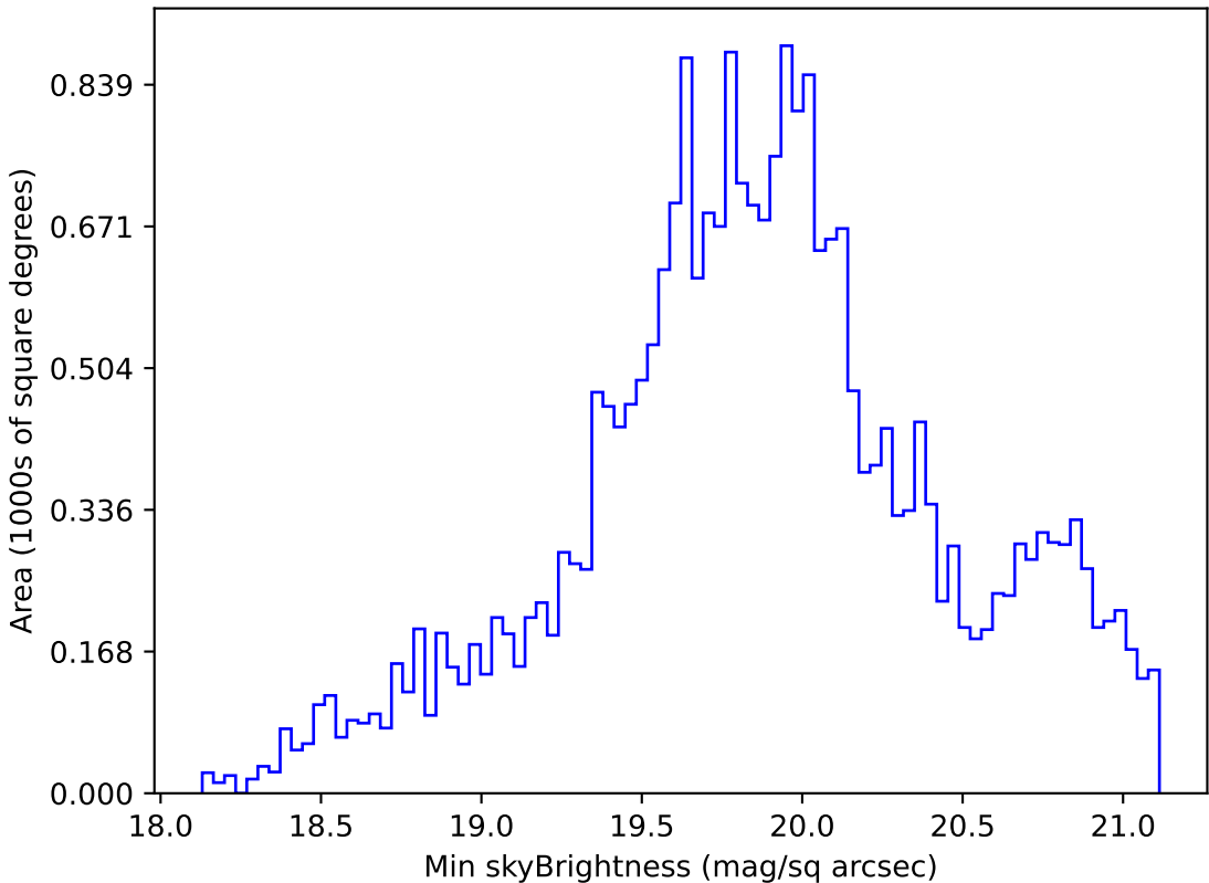
weather_cloudso6v3.4_10yrs Yr 1 r band: Min skyBrightness
