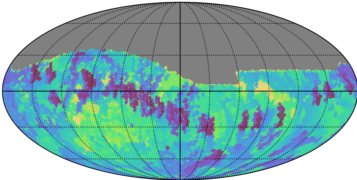
weather_cloudso6v3.4_10yrs Yr 1 i band: Min skyBrightness
