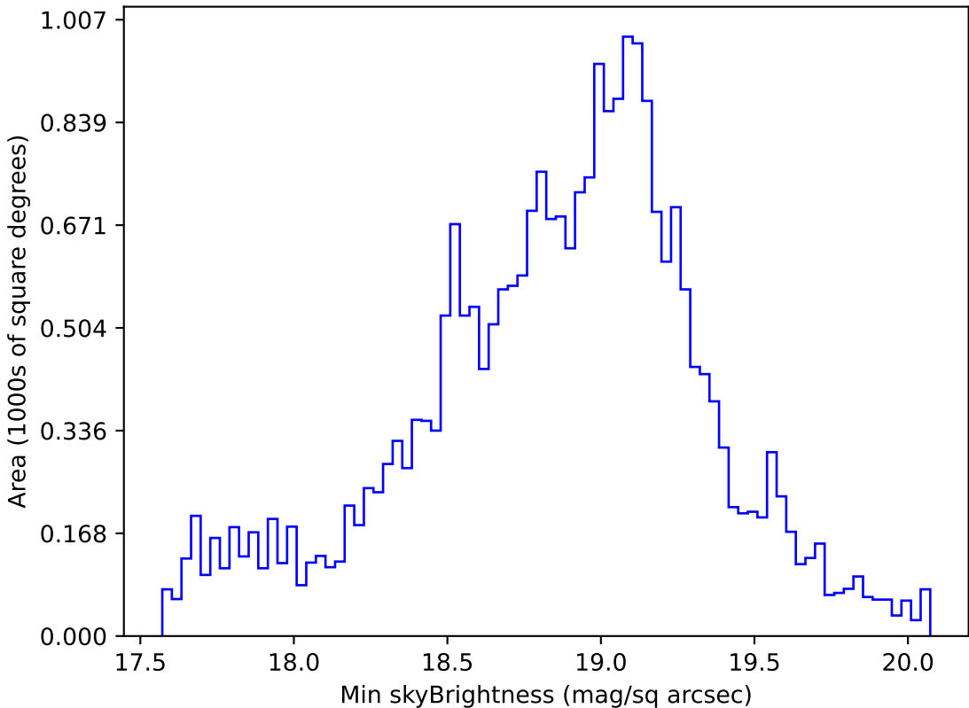
weather_cloudso6v3.4_10yrs Yr 1 i band: Min skyBrightness
