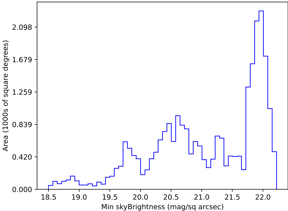
weather_cloudso6v3.4_10yrs Yr 1 g band: Min skyBrightness
