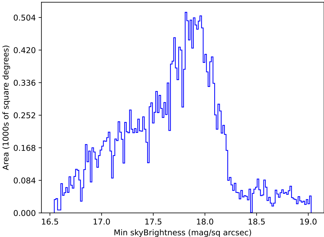
weather_cloudso6v3.4_10yrs Yr 1 all bands: Min skyBrightness
