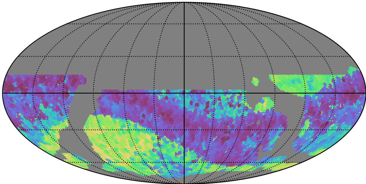
weather_cloudso6v3.4_10yrs WFD z band: Min skyBrightness
