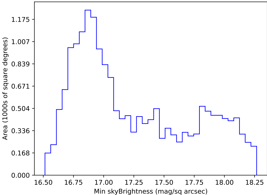
weather_cloudso6v3.4_10yrs WFD z band: Min skyBrightness
