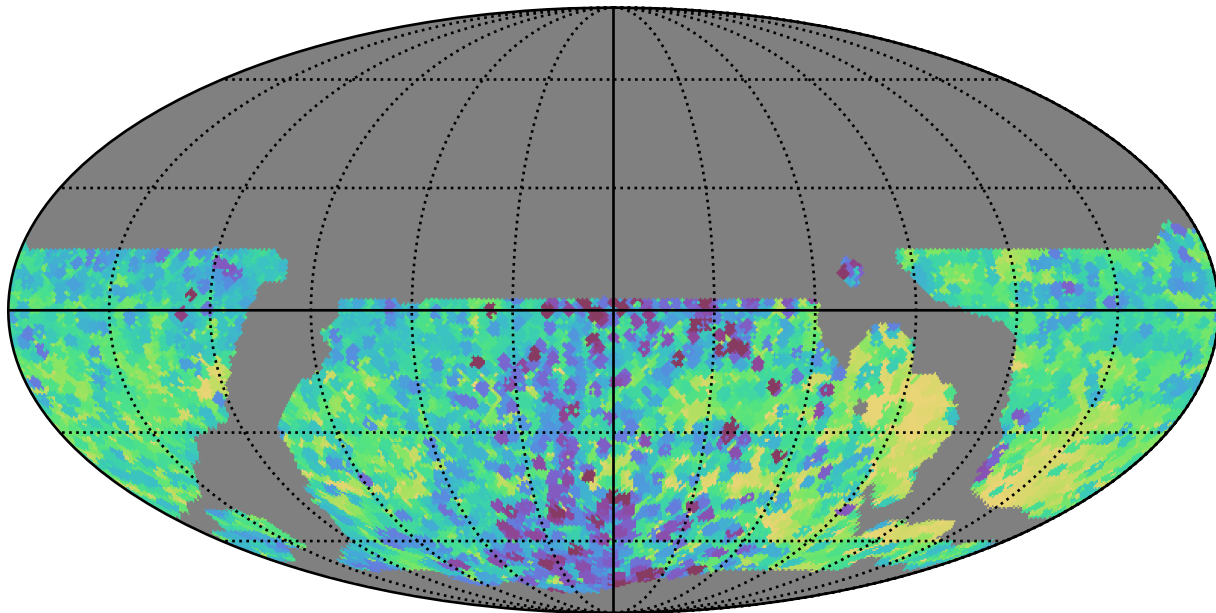
weather_cloudso6v3.4_10yrs WFD y band: Min skyBrightness
