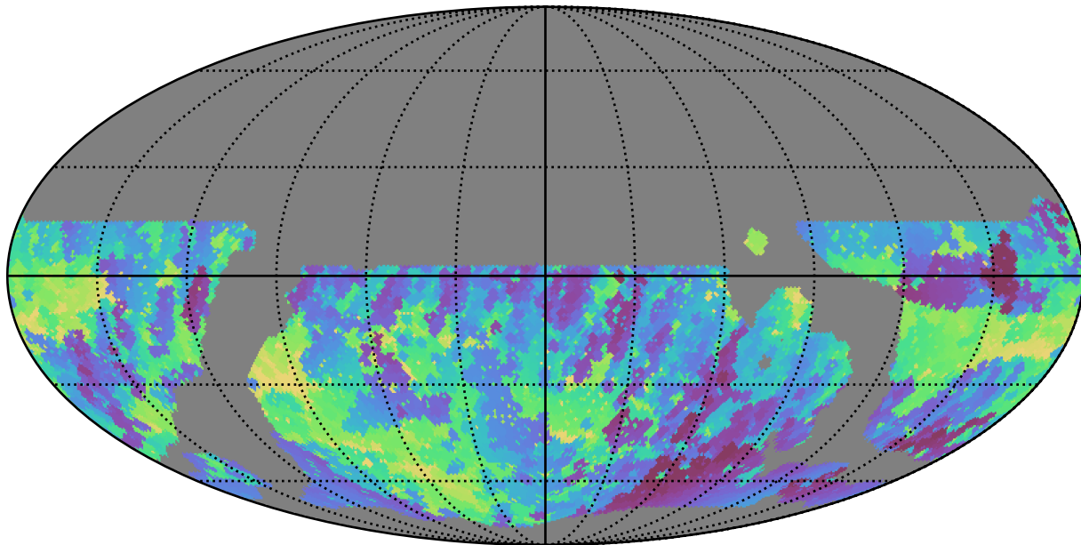
weather_cloudso6v3.4_10yrs WFD r band: Min skyBrightness
