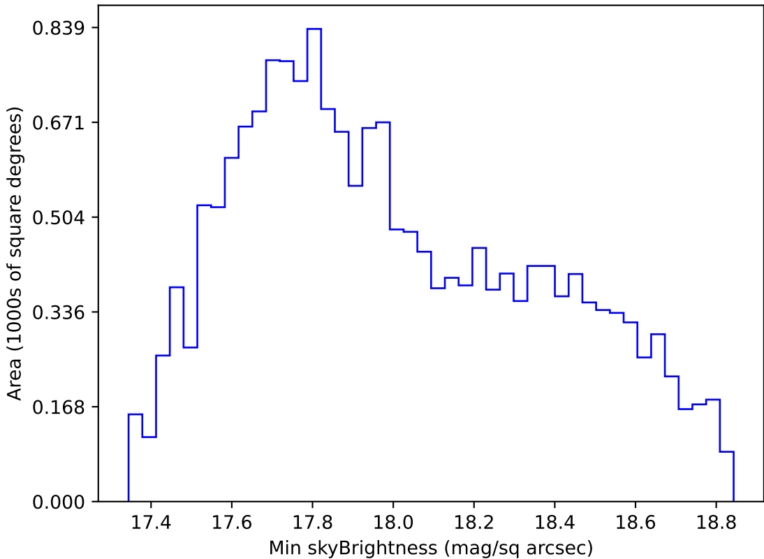
weather_cloudso6v3.4_10yrs WFD i band: Min skyBrightness
