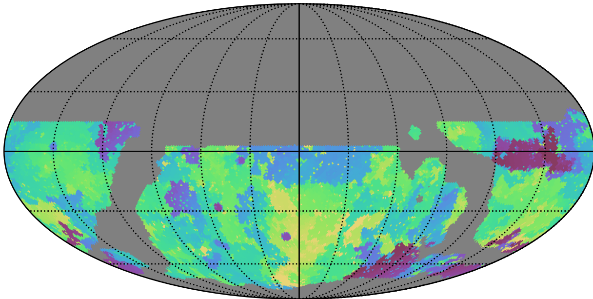
weather_cloudso6v3.4_10yrs WFD g band: Min skyBrightness
