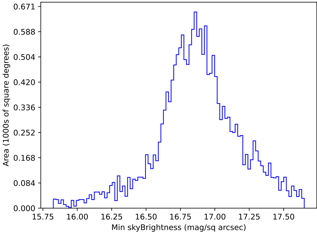
weather_cloudso6v3.4_10yrs WFD all bands: Min skyBrightness
