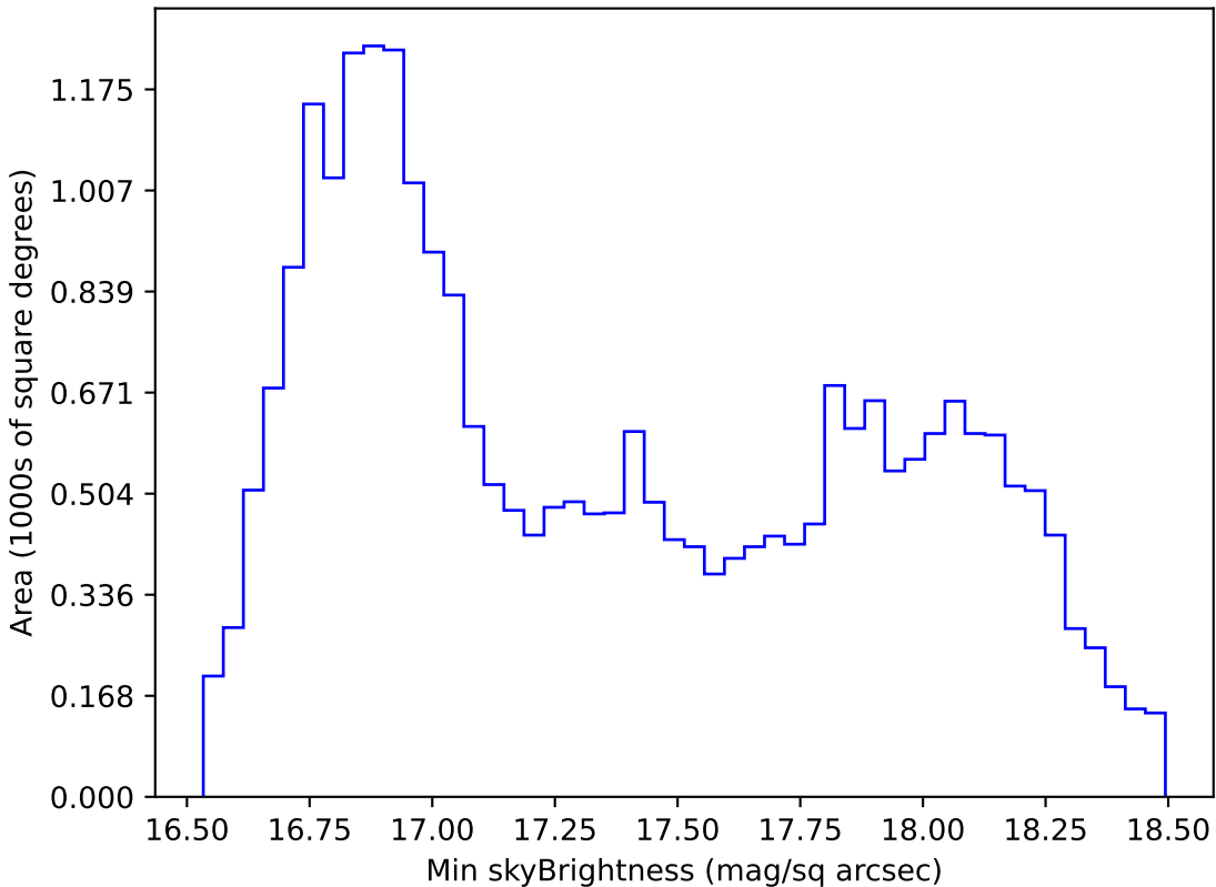
weather_cloudso6v3.4_10yrs All sky z band: Min skyBrightness
