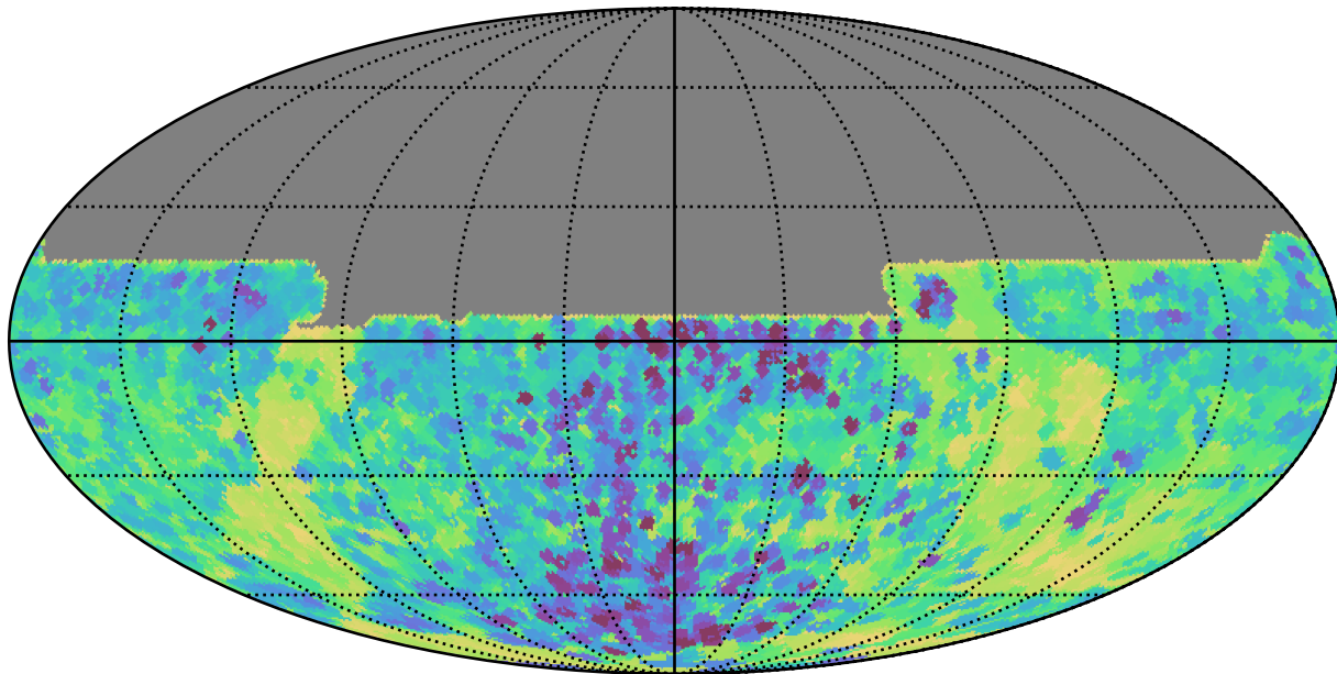
weather_cloudso6v3.4_10yrs All sky y band: Min skyBrightness
