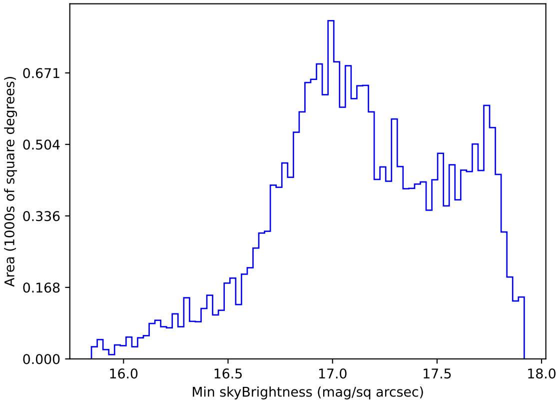
weather_cloudso6v3.4_10yrs All sky y band: Min skyBrightness
