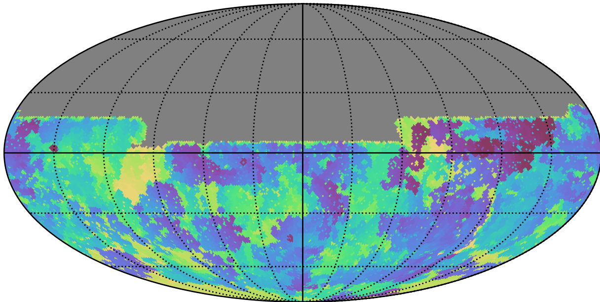
weather_cloudso6v3.4_10yrs All sky u band: Min skyBrightness
