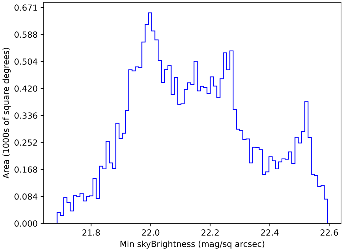
weather_cloudso6v3.4_10yrs All sky u band: Min skyBrightness
