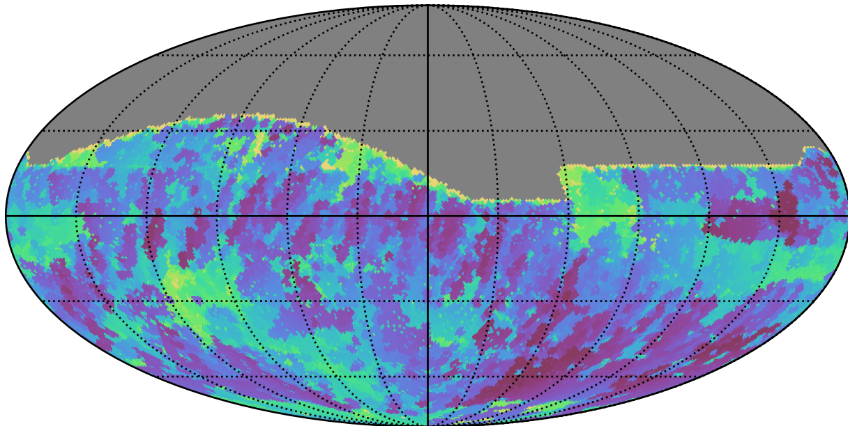
weather_cloudso6v3.4_10yrs All sky r band: Min skyBrightness
