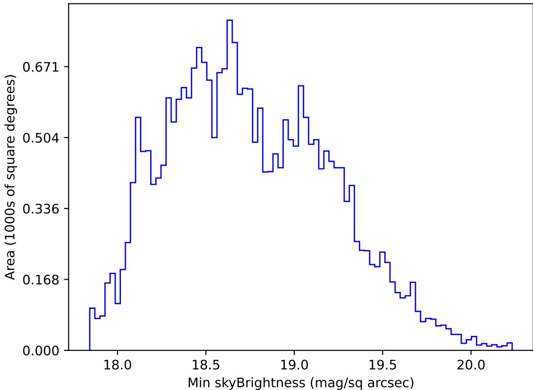
weather_cloudso6v3.4_10yrs All sky r band: Min skyBrightness
