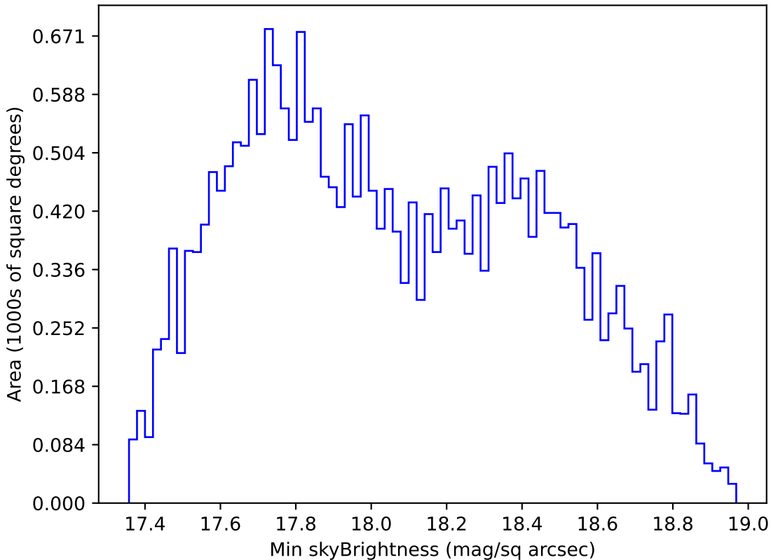
weather_cloudso6v3.4_10yrs All sky i band: Min skyBrightness
