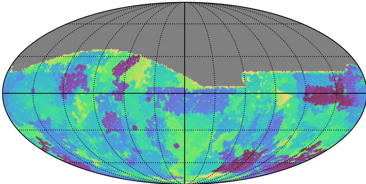
weather_cloudso6v3.4_10yrs All sky g band: Min skyBrightness
