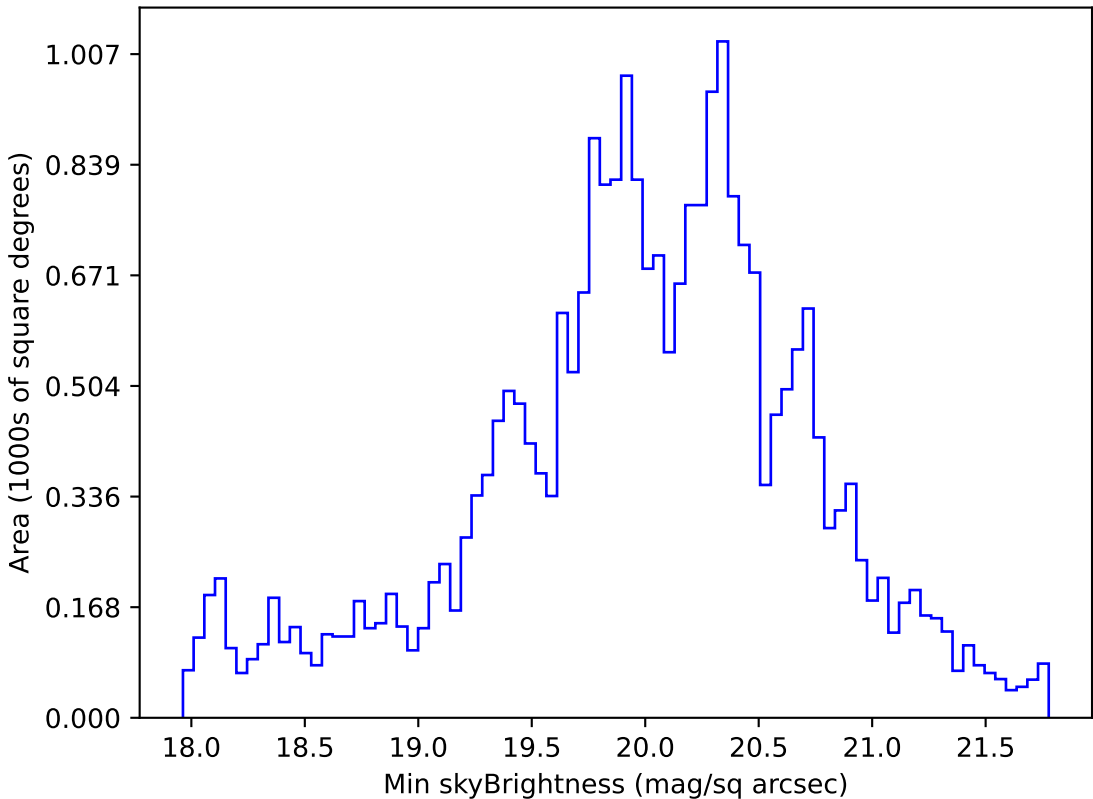
weather_cloudso6v3.4_10yrs All sky g band: Min skyBrightness
