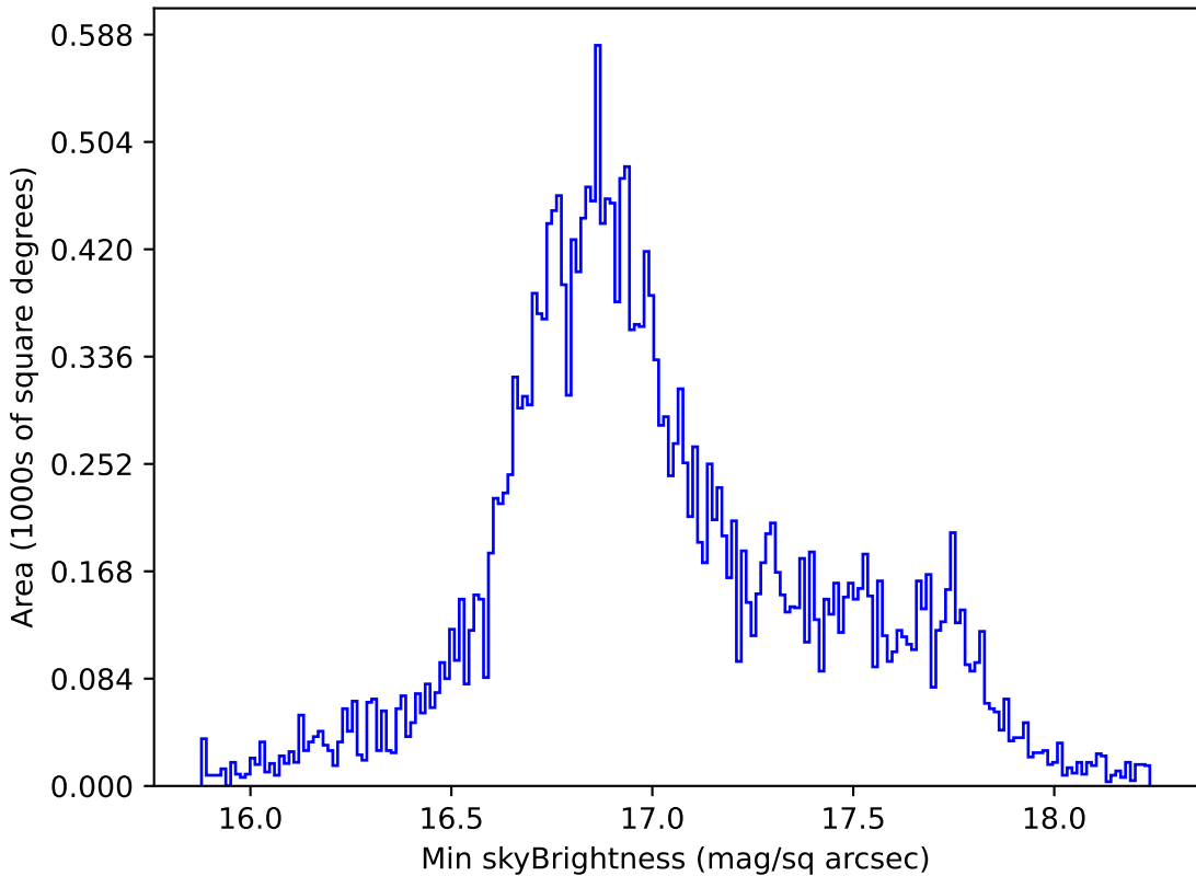
weather_cloudso6v3.4_10yrs All sky all bands: Min skyBrightness
