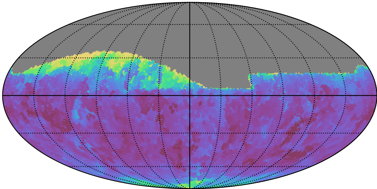
weather_cloudso6v3.4_10yrs Yr 1 all bands: Min seeingGeom
