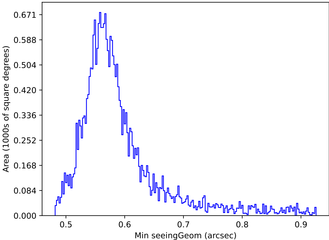
weather_cloudso6v3.4_10yrs Yr 1 all bands: Min seeingGeom
