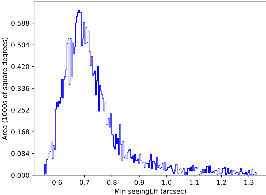
weather_cloudso6v3.4_10yrs Yr 1 z band: Min seeingEff
