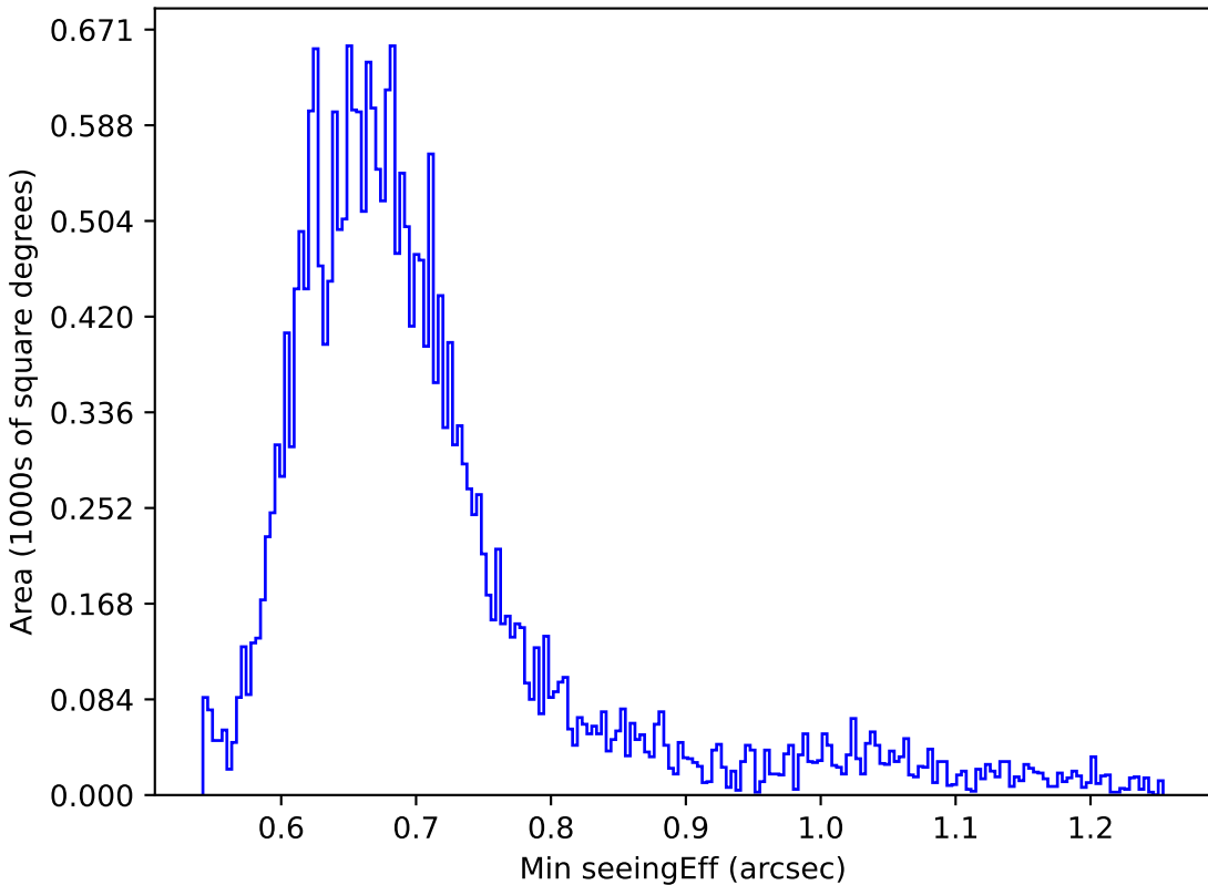
weather_cloudso6v3.4_10yrs Yr 1 r band: Min seeingEff
