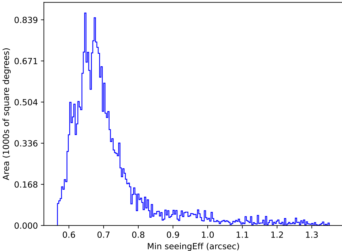
weather_cloudso6v3.4_10yrs Yr 1 i band: Min seeingEff
