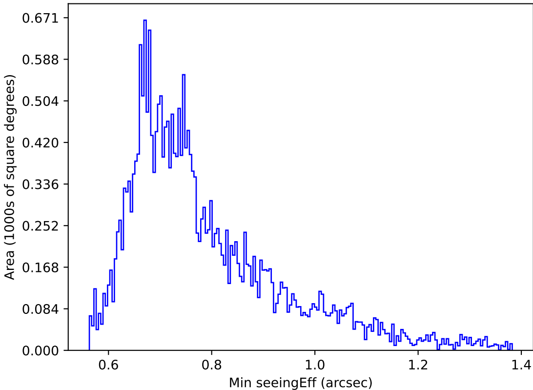
weather_cloudso6v3.4_10yrs Yr 1 g band: Min seeingEff
