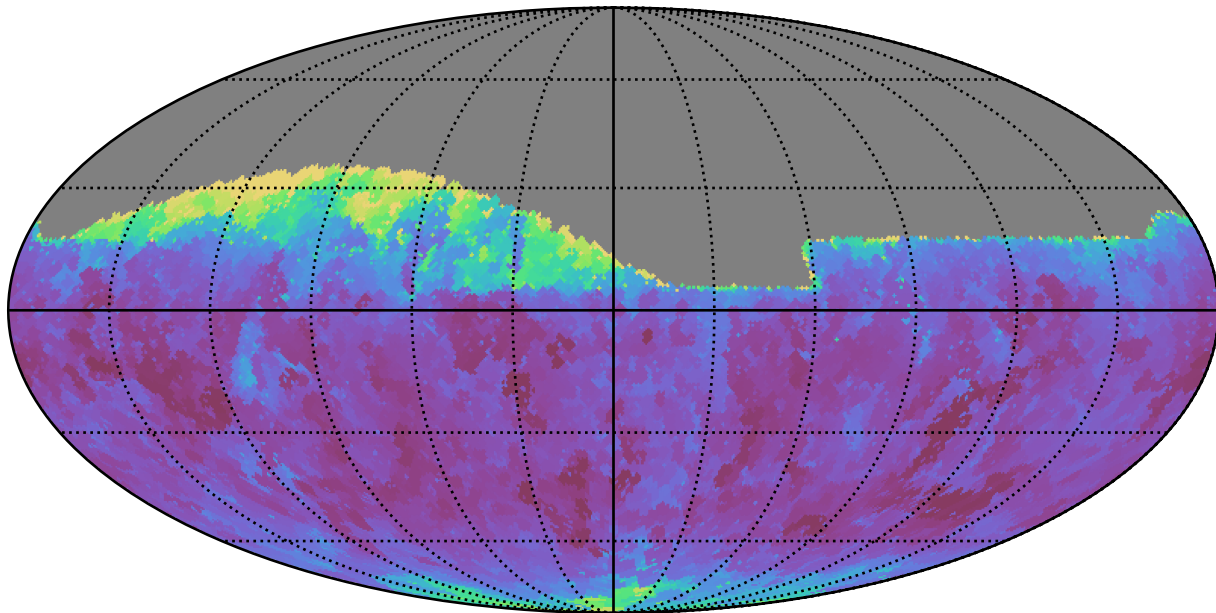
weather_cloudso6v3.4_10yrs Yr 1 all bands: Min seeingEff
