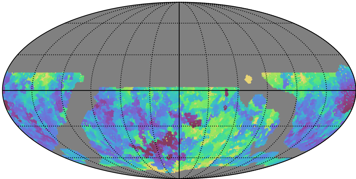
weather_cloudso6v3.4_10yrs WFD u band: Min seeingEff
