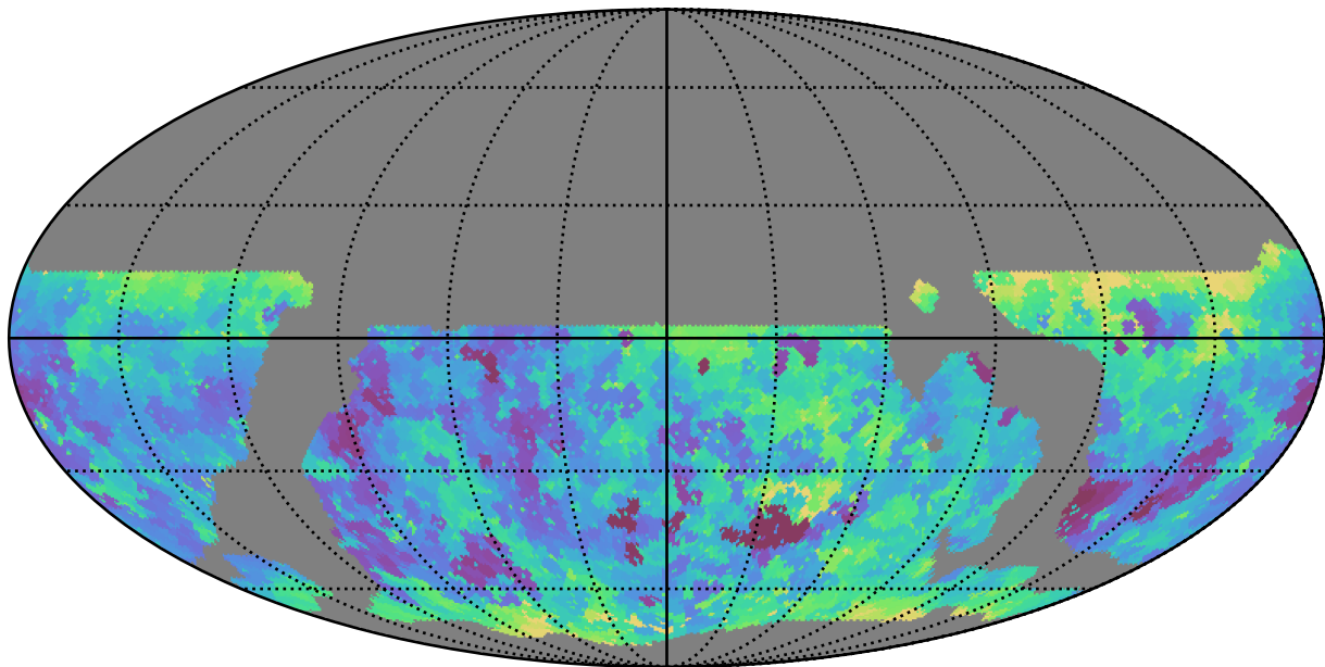
weather_cloudso6v3.4_10yrs WFD g band: Min seeingEff
