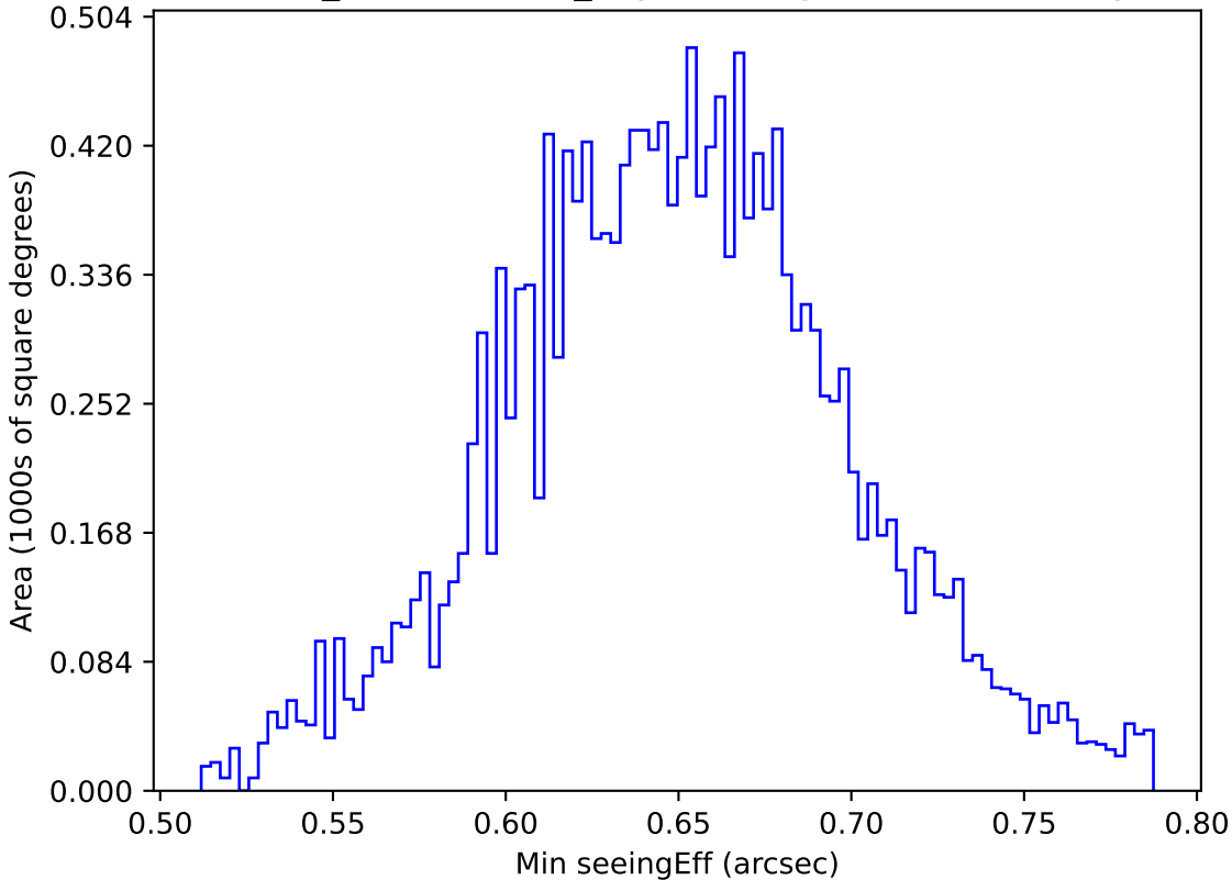
weather_cloudso6v3.4_10yrs WFD g band: Min seeingEff
