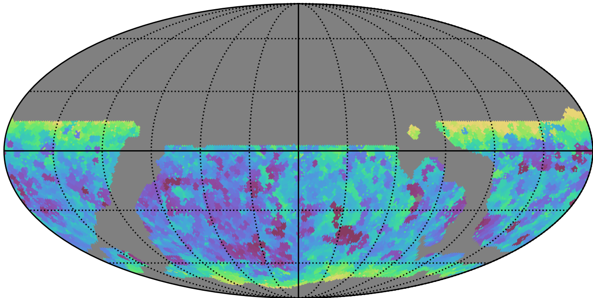
weather_cloudso6v3.4_10yrs WFD all bands: Min seeingEff
