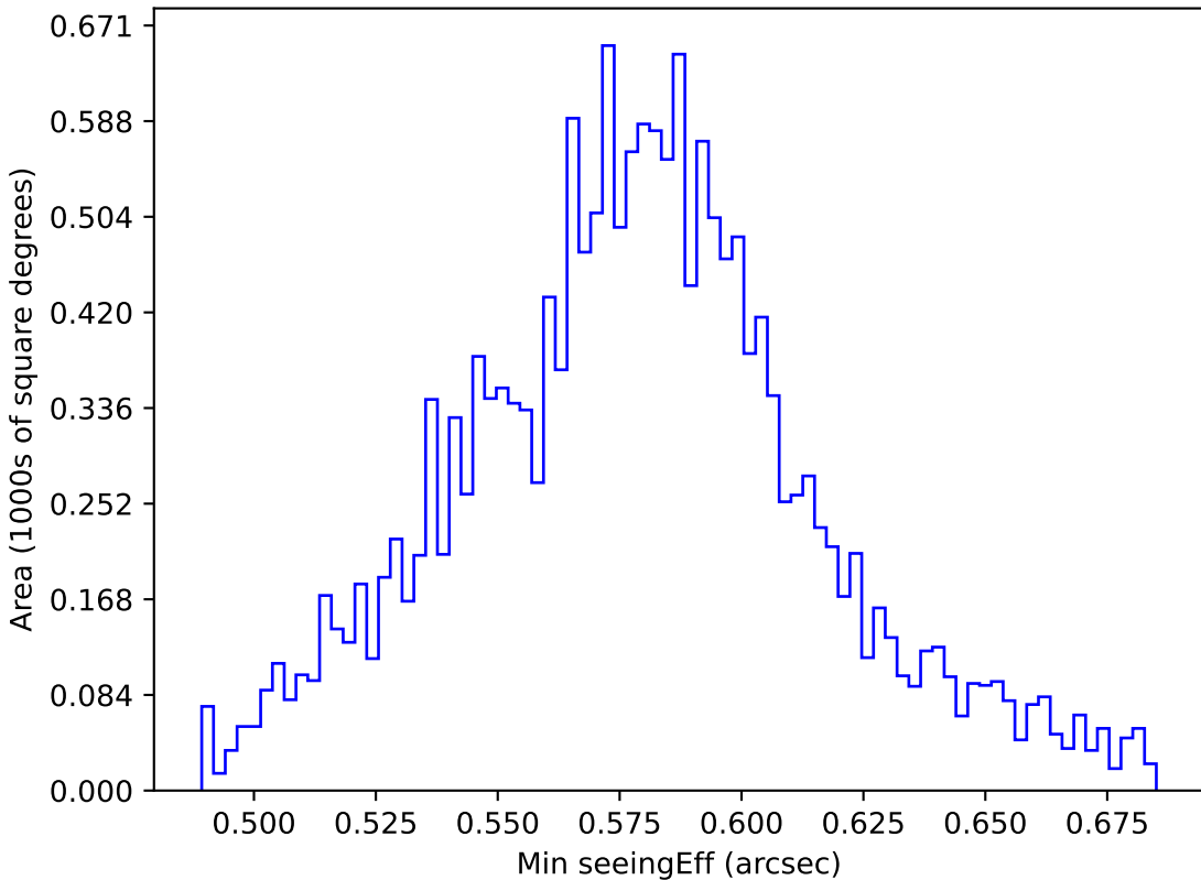
weather_cloudso6v3.4_10yrs WFD all bands: Min seeingEff
