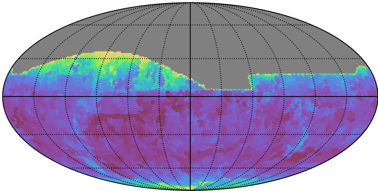
weather_cloudso6v3.4_10yrs All sky z band: Min seeingEff
