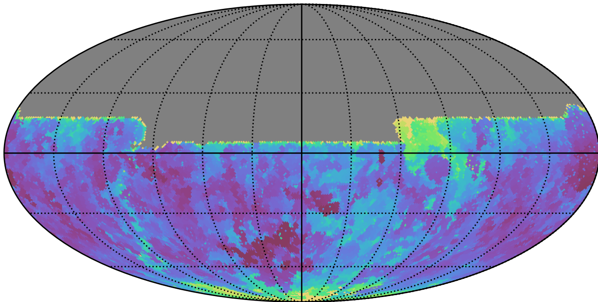
weather_cloudso6v3.4_10yrs All sky u band: Min seeingEff
