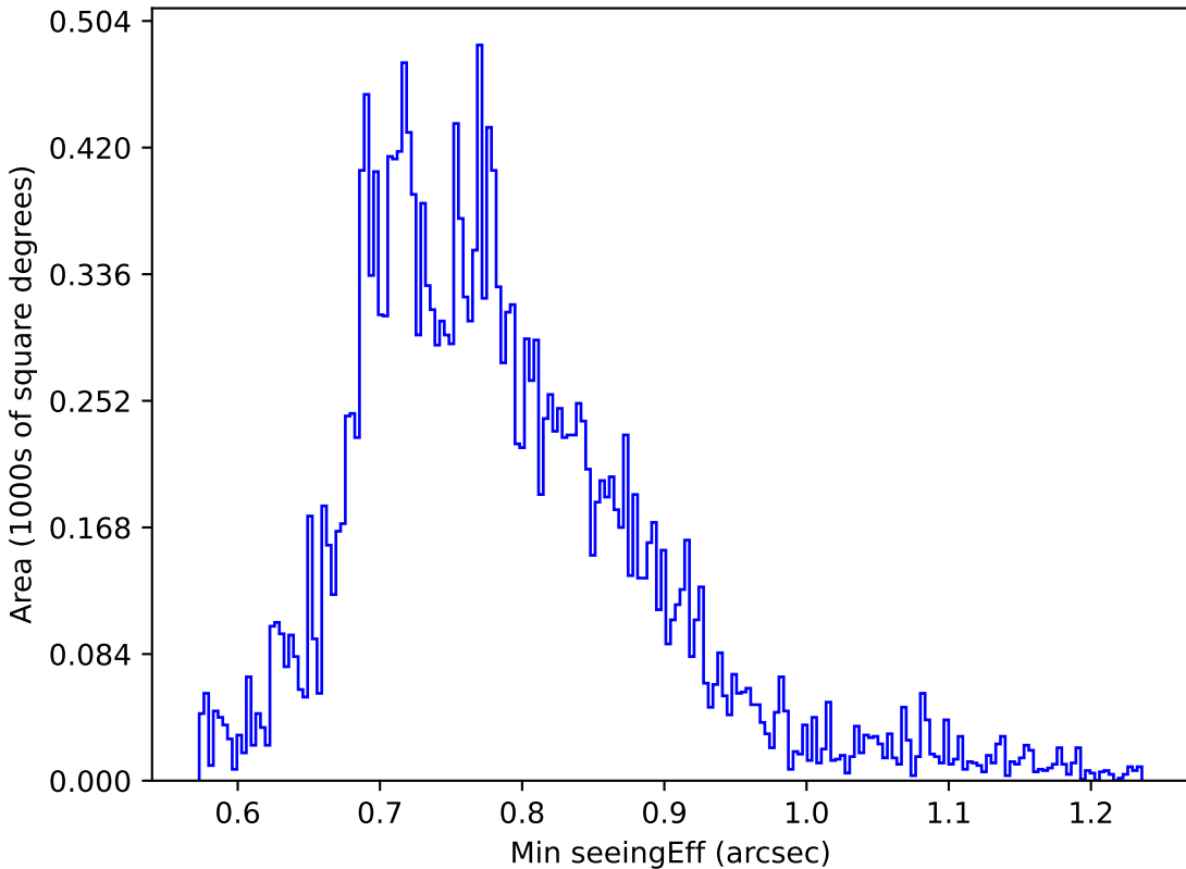
weather_cloudso6v3.4_10yrs All sky u band: Min seeingEff
