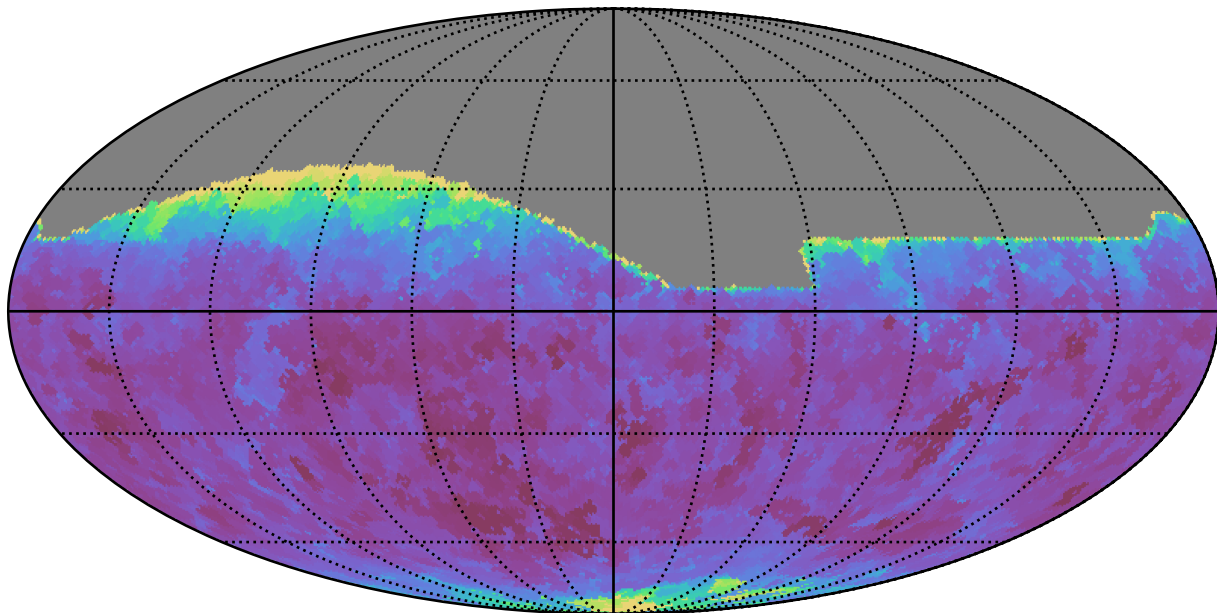
weather_cloudso6v3.4_10yrs All sky r band: Min seeingEff
