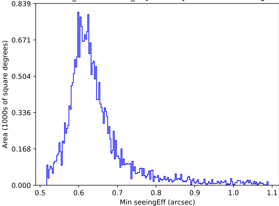
weather_cloudso6v3.4_10yrs All sky r band: Min seeingEff
