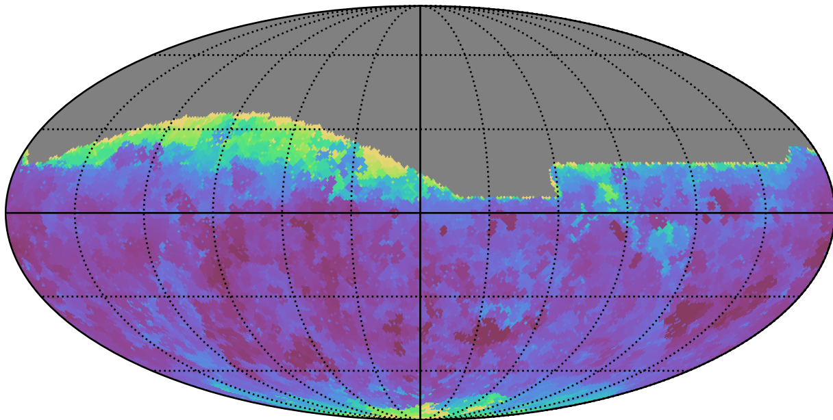
weather_cloudso6v3.4_10yrs All sky g band: Min seeingEff
