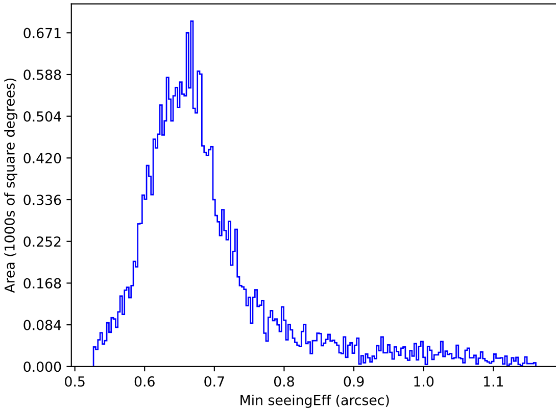
weather_cloudso6v3.4_10yrs All sky g band: Min seeingEff
