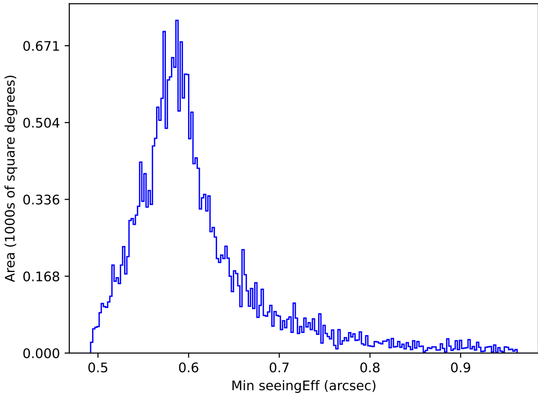
weather_cloudso6v3.4_10yrs All sky all bands: Min seeingEff
