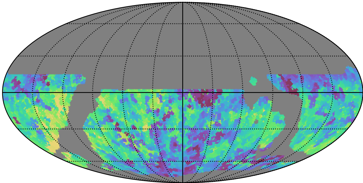
weather_cloudso6v3.4_10yrs WFD all bands: Min saturation_mag
