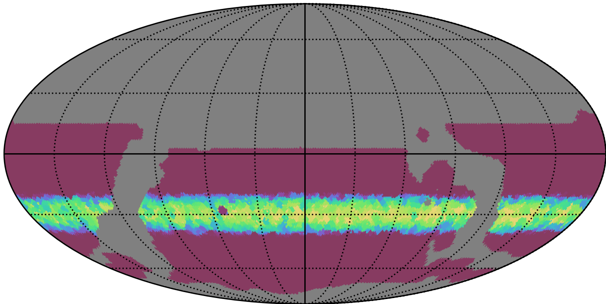
weather_cloudso6v3.4_10yrs WFD all bands: Min normairmass
