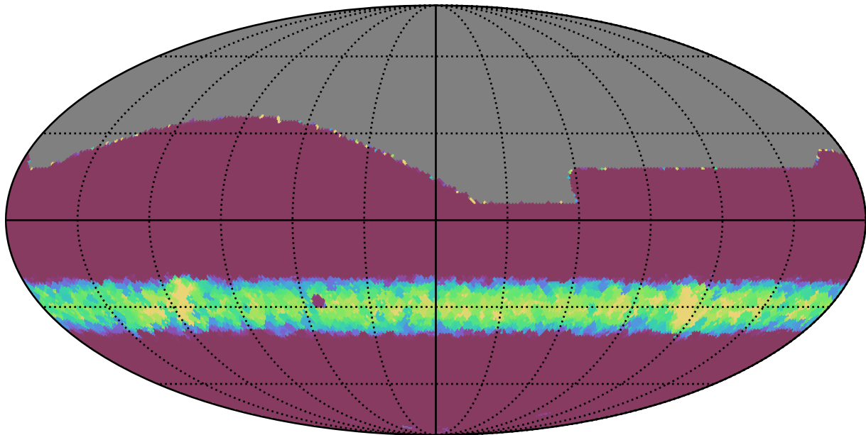
weather_cloudso6v3.4_10yrs All sky all bands: Min normairmass
